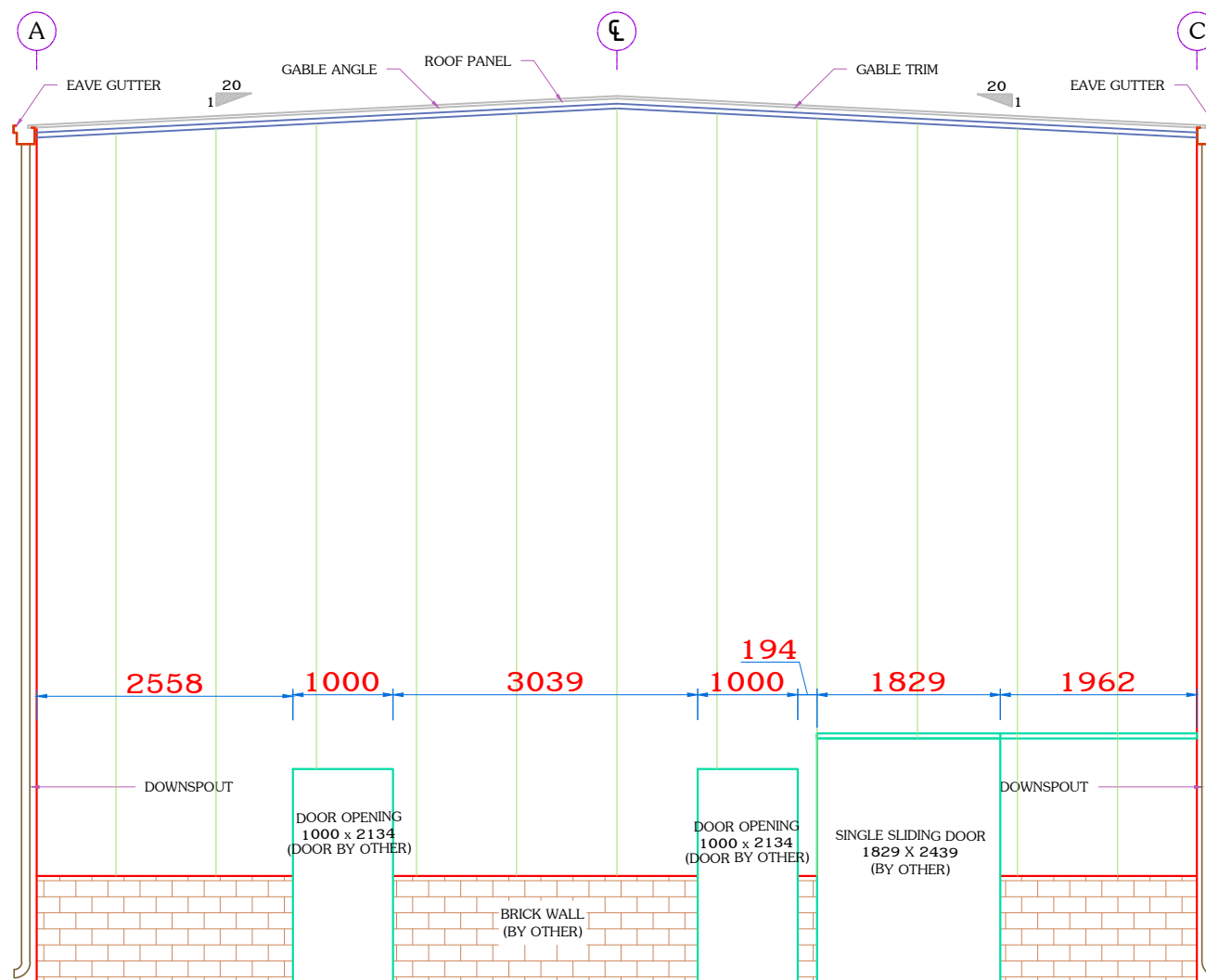
END WALL SHEETING @ GRID-1
